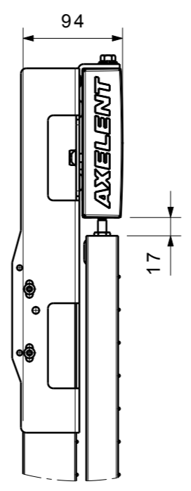
A (1:5)
