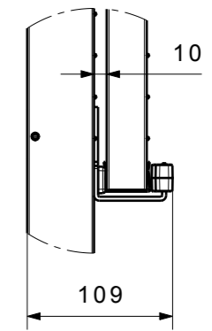
B (1:5)
